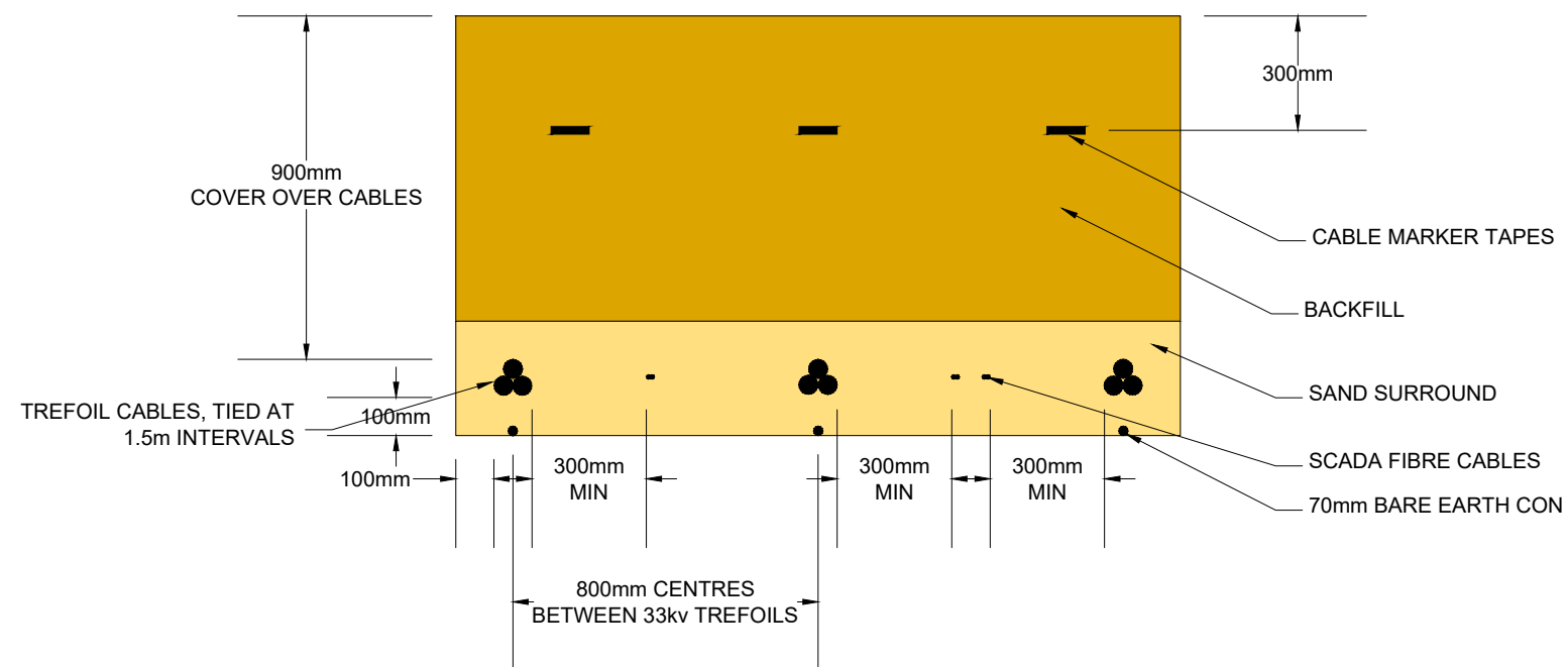
CABLE TRENCH SECTION SHOWING DOUBLE CIRCUIT
