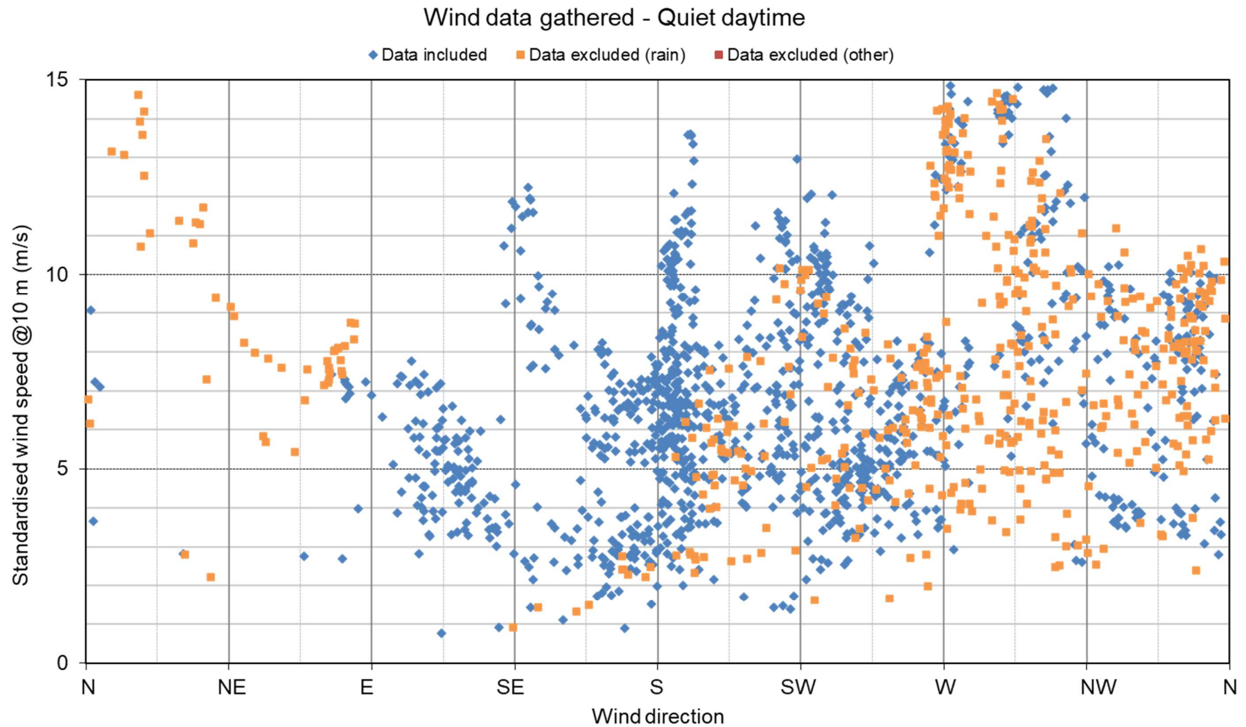
Graph 13-1: Wind Data for MP1, MP2 and MP4 – Quiet Daytime Periods
