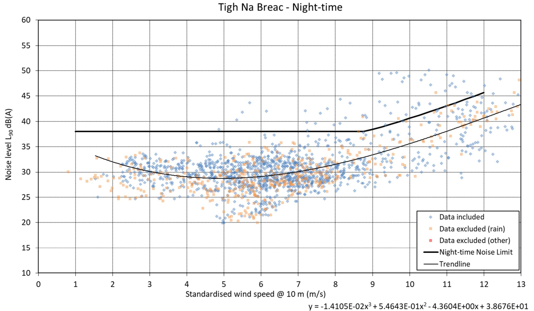
Graph 13-9: Noise and Wind Data at MP3 Calgary Beg – Quiet Day-time Periods
